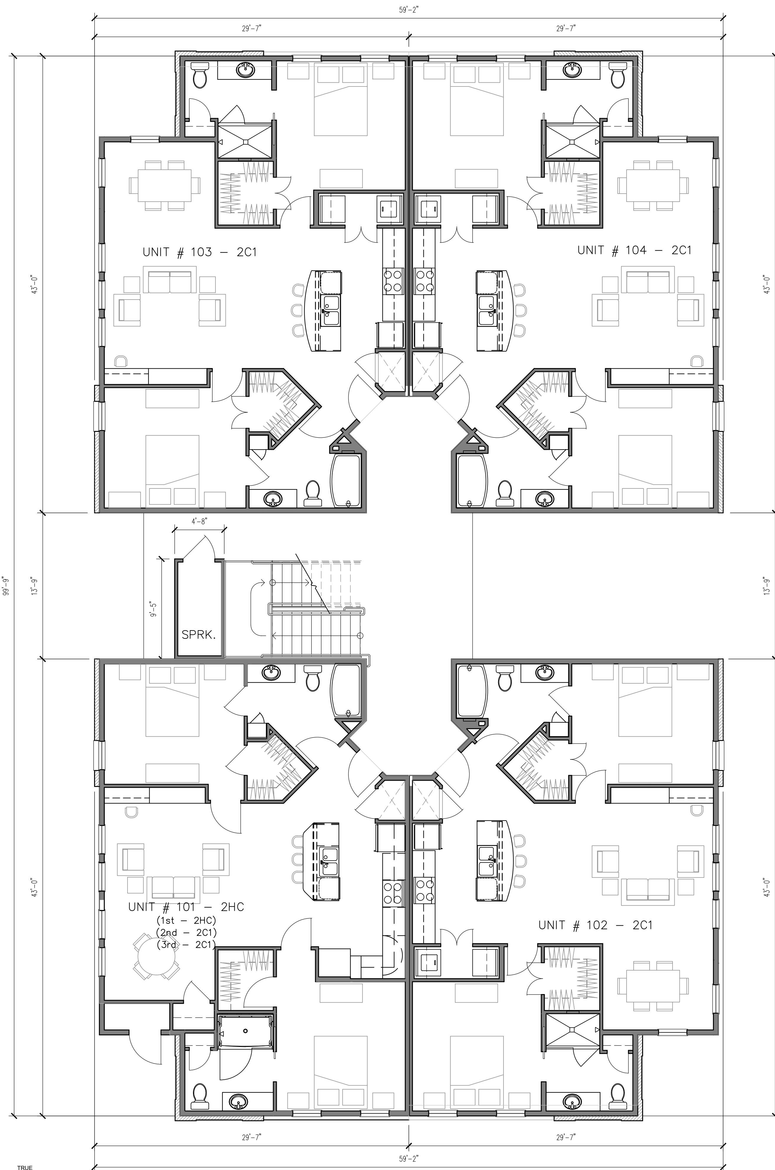
1 BUILDING 1 PLAN - 1st, 2nd & 3rd FLOOR PLANS A2.01 SCALE: 3/16" = 1'-0"
